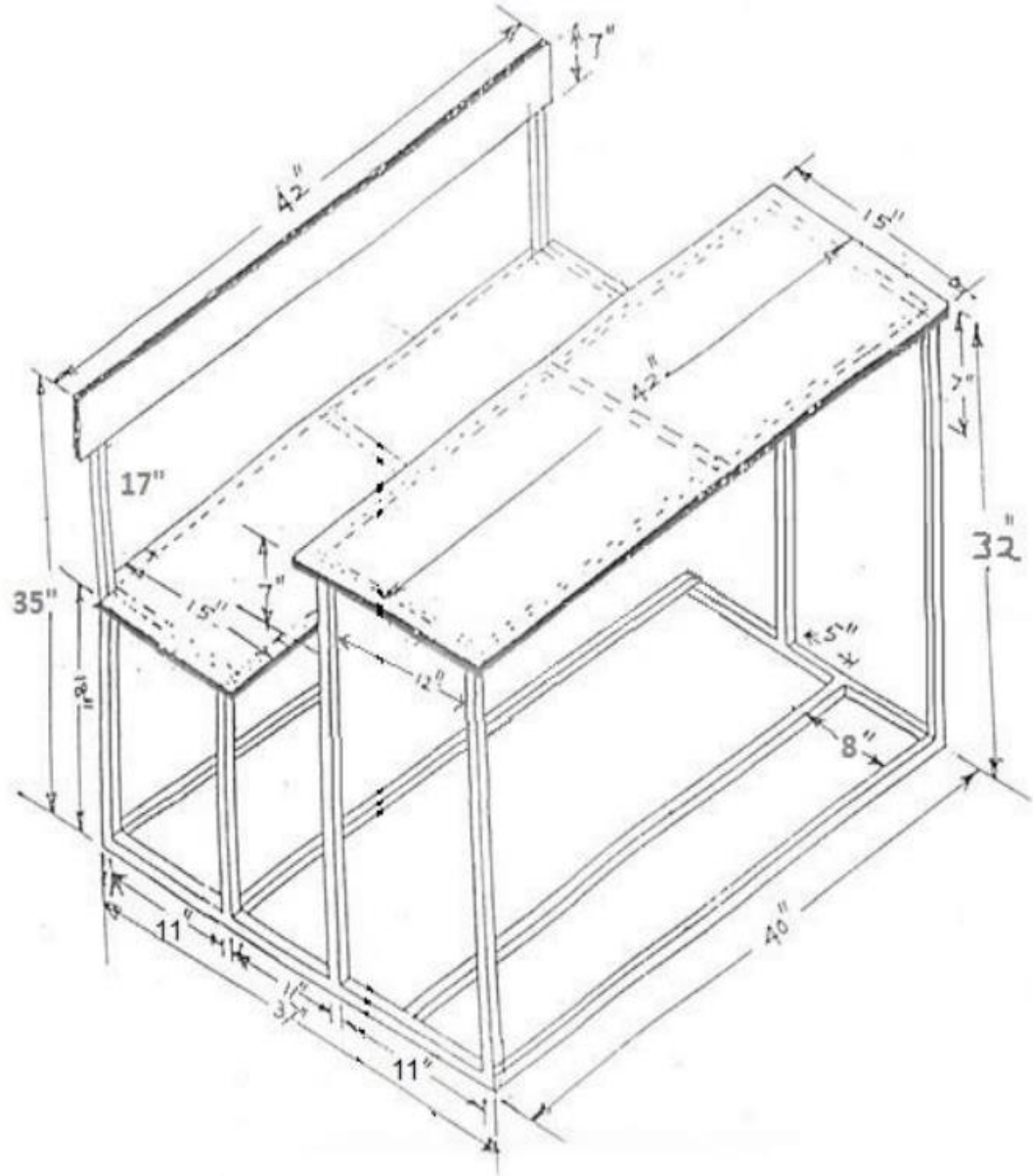
COMPACT DESK-CUM-BENCH (DUAL DESK) SIZE - 42" x 37" x 32"
